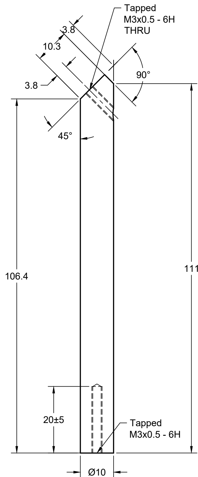
RIGHT VIEW
